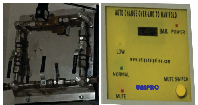
Automatic Changeover from O2 Liquid Tank, Emergence Gas Manifold to Main Gas Manifold & Vice-Versa
