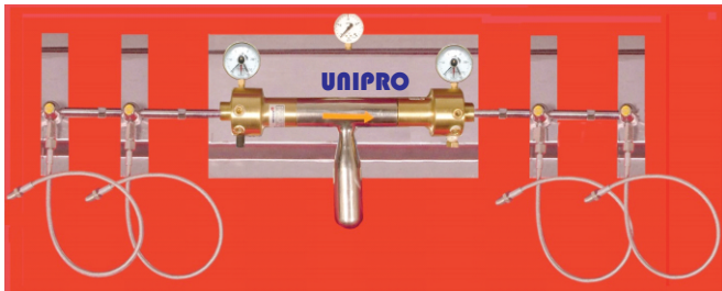
SS 304 2+2 Oxygen Manifold with Semi Automatic Changeover
